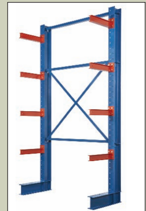
Single-sided I-Beam Cantilever Rack
