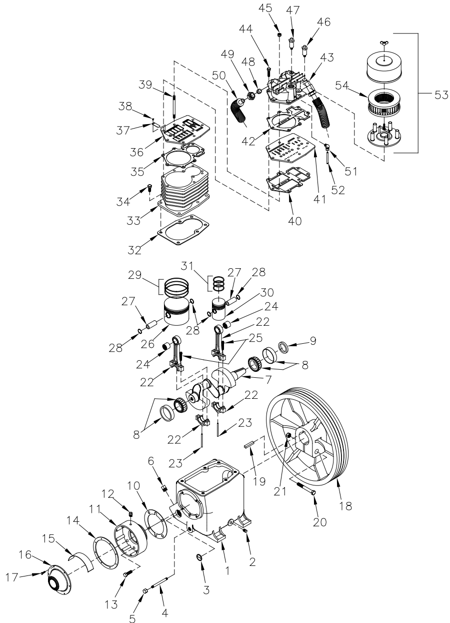
C292-A (Ref. Drawing)
