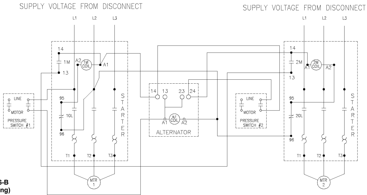
Figure 1-2 Wiring Diagram
