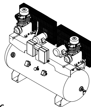
C286-C (Ref. Drawing)
