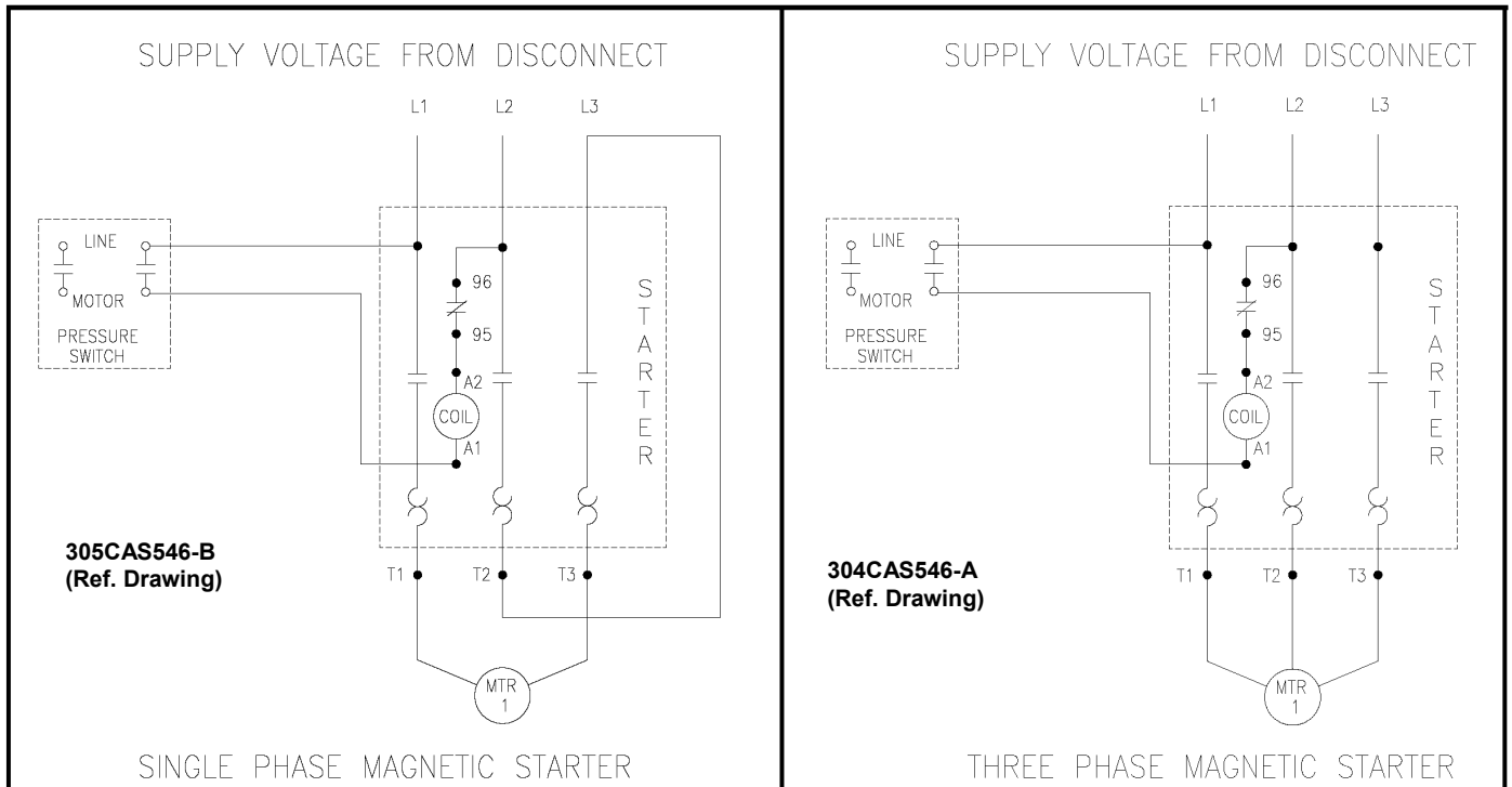
Figure 1-1 Wiring Diagram
