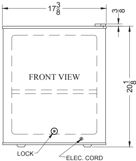
FRONT VIEW LR021WWW/0 LF021WWW/0
