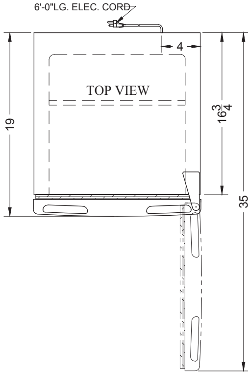
TOP VIEW LR021WWW/0 LF021WWW/0
