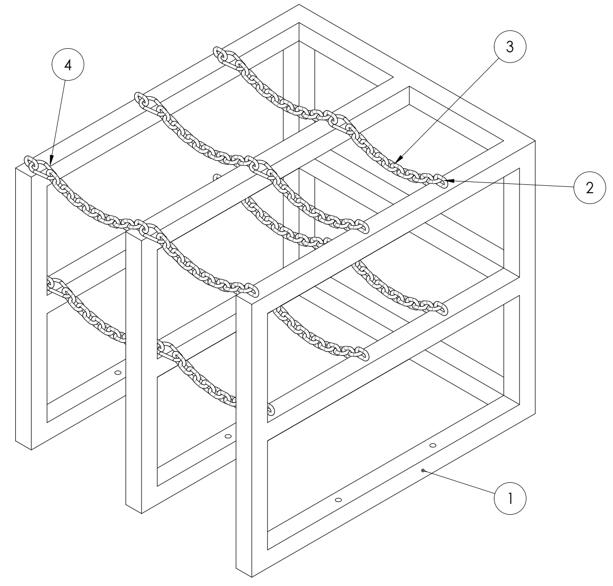
ISOMETRIC SCALE 1:8
