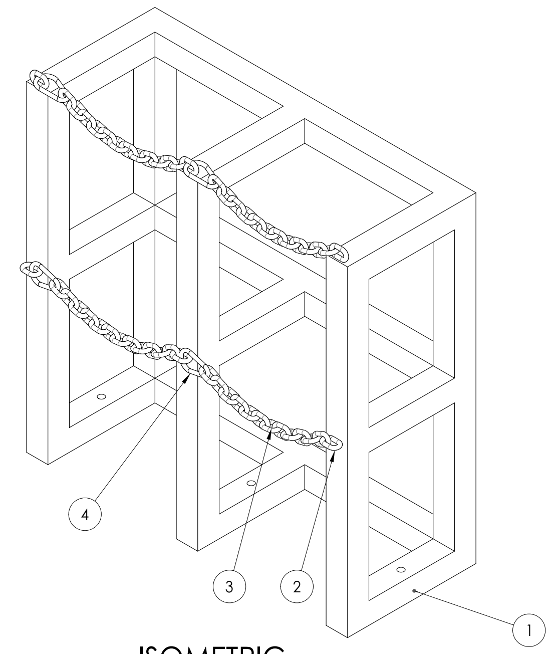
ISOMETRIC SCALE 1:6
