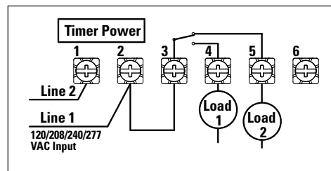
ET1715 configured for SPDT load switching
