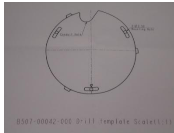
Drill Template
