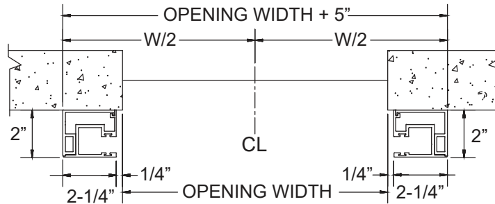
EXTRUDED ALUMINUM GUIDE FACE OF WALL DETAIL
