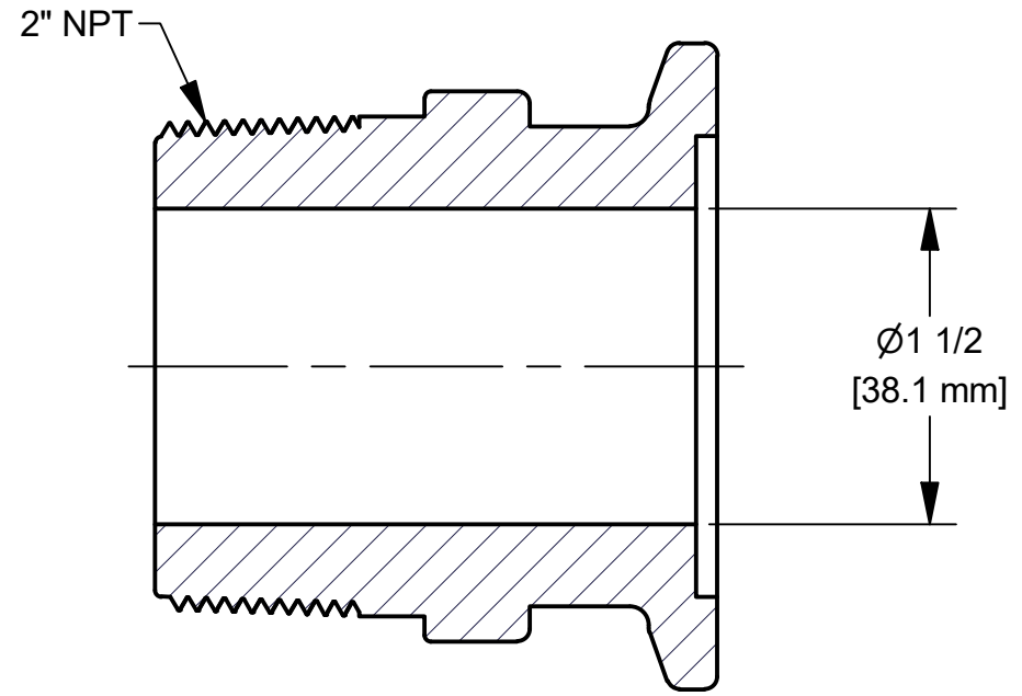
SECTION A-A SCALE 1
