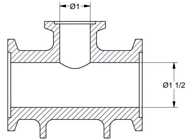
SECTION E-E SCALE 1 : 1
