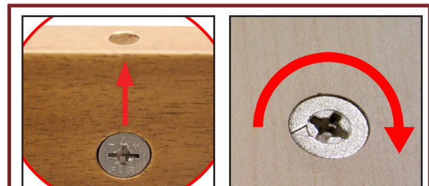
FIGURE 1: To open Cam Lock, point arrow toward Cam Pin Hole. To close and lock Cam, turn clockwise
