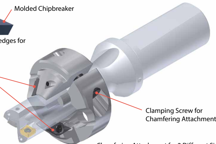
Chamfering Attachment for 2 Different Size Drills
