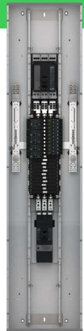
800A NF MB Panelboard with 600A SFB
