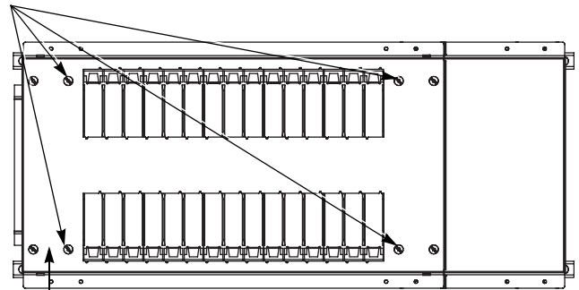
Deadfront assembly
